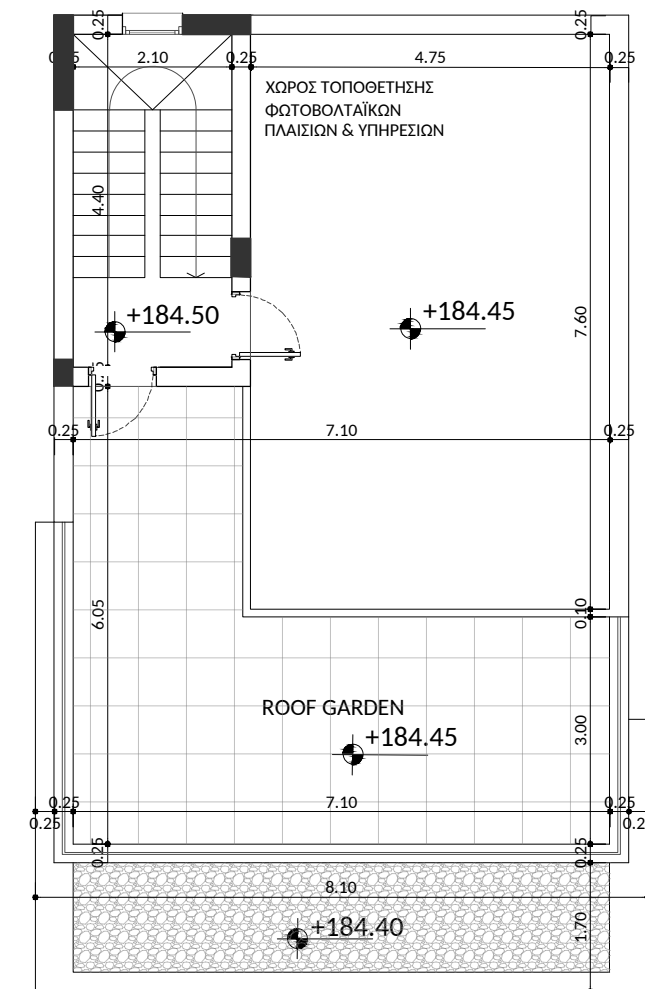
ROOF
