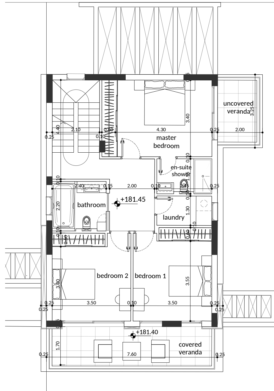
FIRST FLOOR
